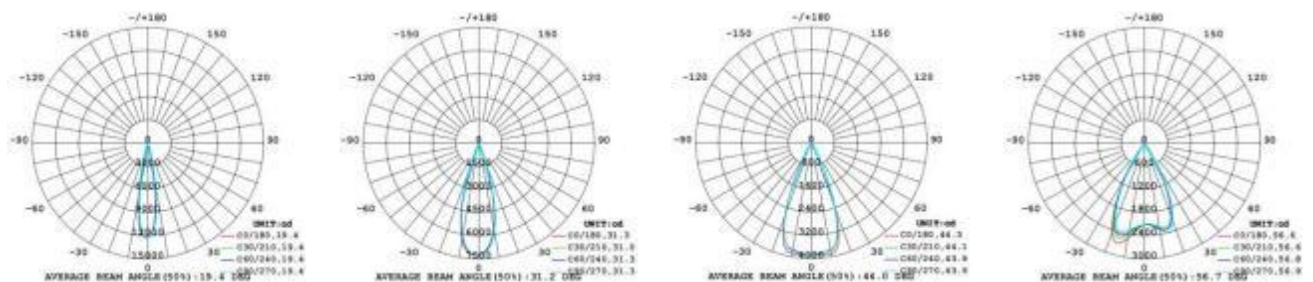
Luminous intensity distribution diagram
